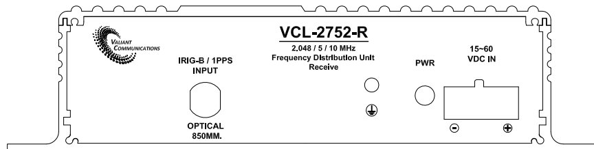
Front View
